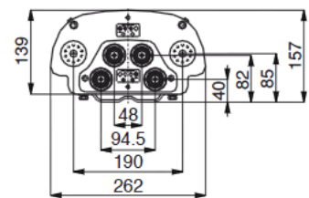
Bottom view (Dimensions refer to radome)
