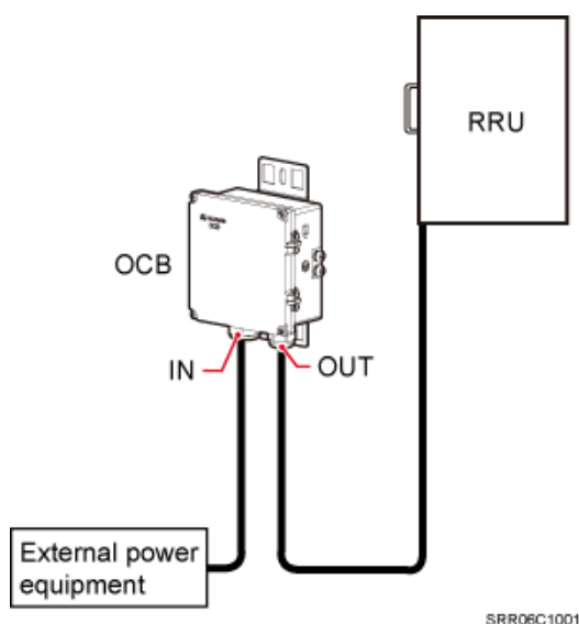
Figure 4-2 Application scenario of an OCB
