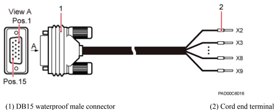
Figure 3-4 Alarm cable
