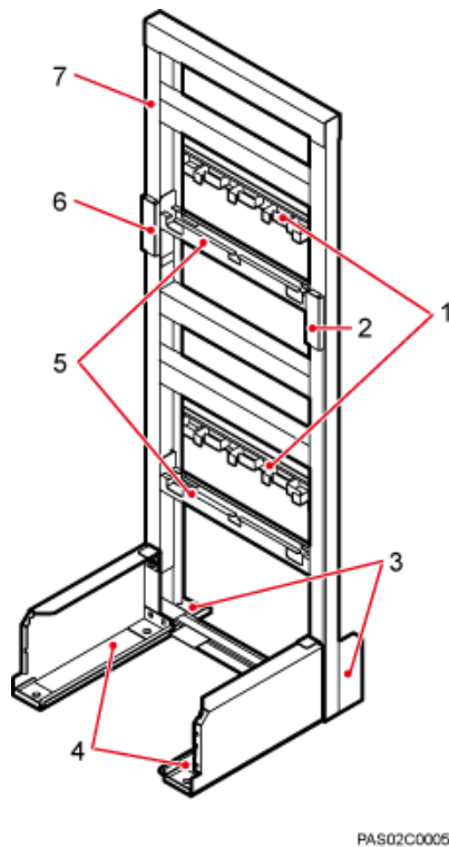
Figure 4-1 IFS06
