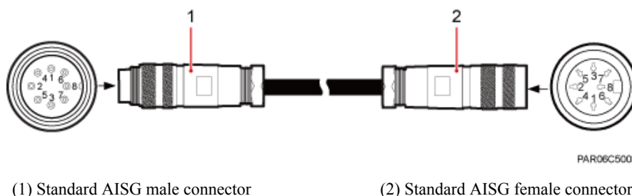
Figure 3-12 AISG extension cable
