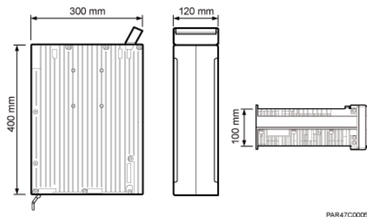
Figure 2-2 RRU dimensions
