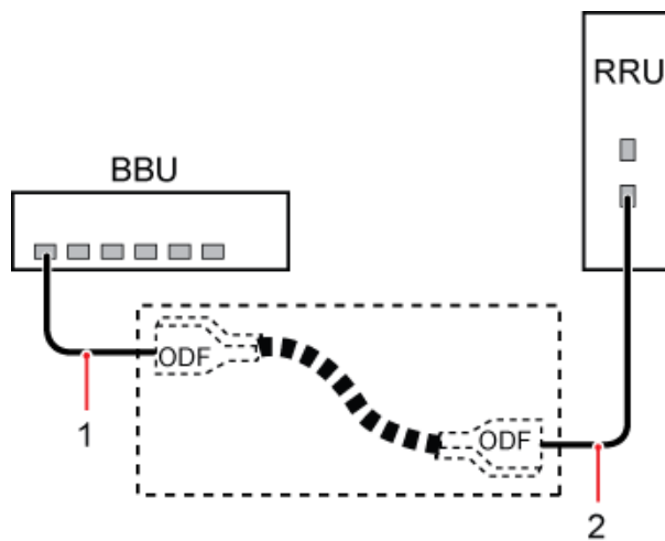
Figure 3-8 Connection of the single-mode pigtail
