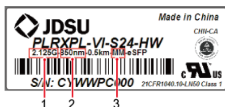
Figure 2-6 Label on an optical module
