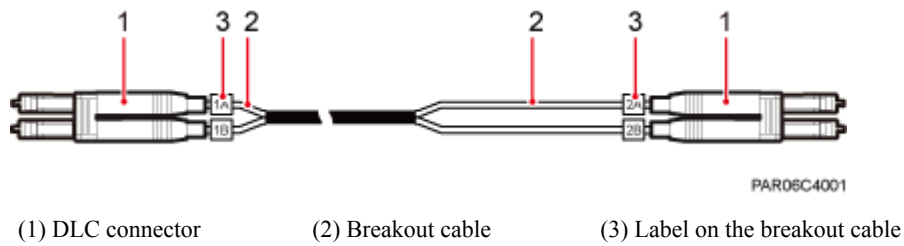
Figure 3-5 Multimode fiber optic cable
