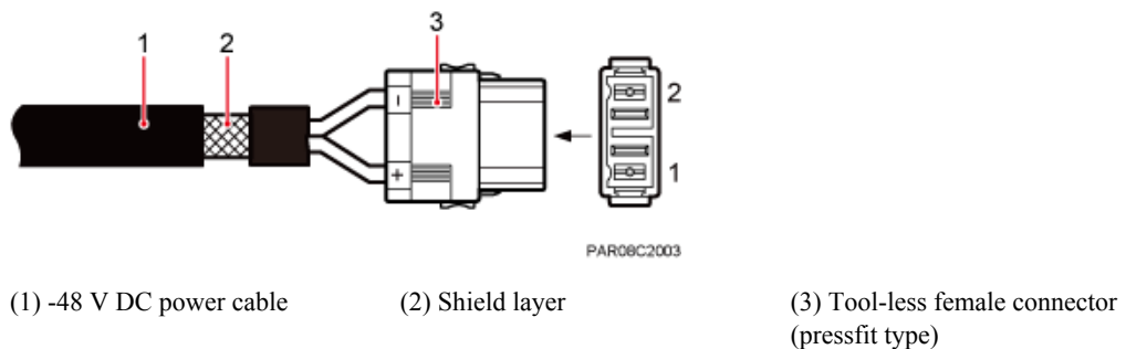
Figure 3-3 RRU power cable
