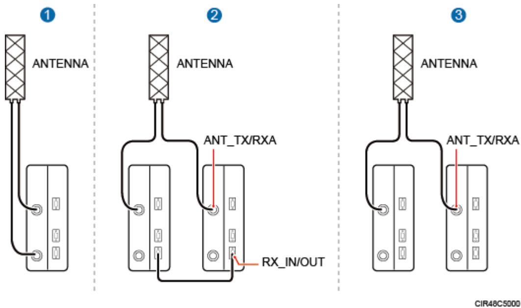
Figure 4-1 RF cable connections for the RRU
