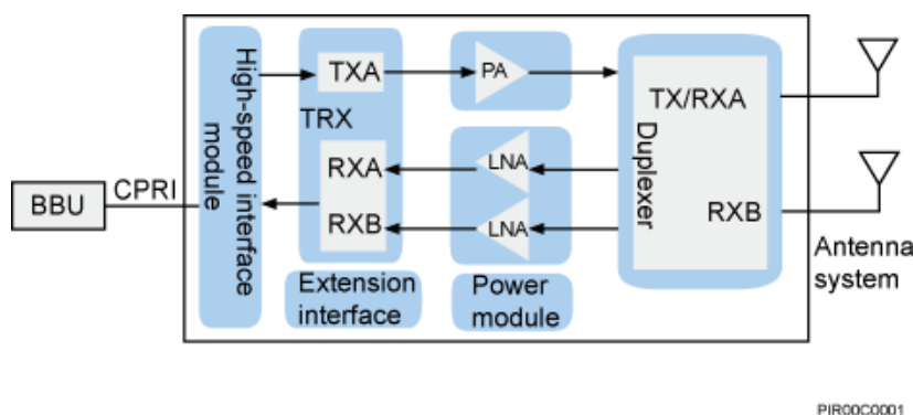
Figure 2-3 Function structure of the RRU
