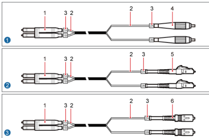
Figure 3-7 Single-mode pigtail
