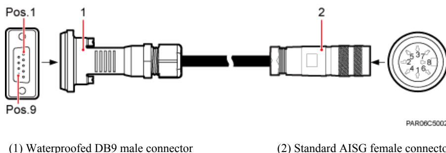
Figure 3-11 AISG multi-wire cable
