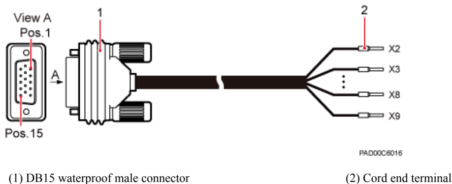
Figure 3-4 Alarm cable
