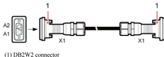
Figure 3-10 Inter-RRU RF cable
