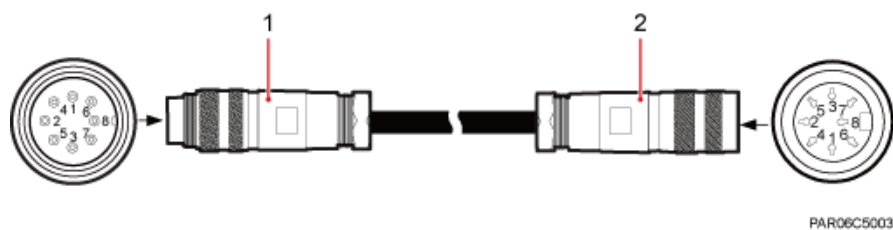
Figure 3-12 AISG extension cable
