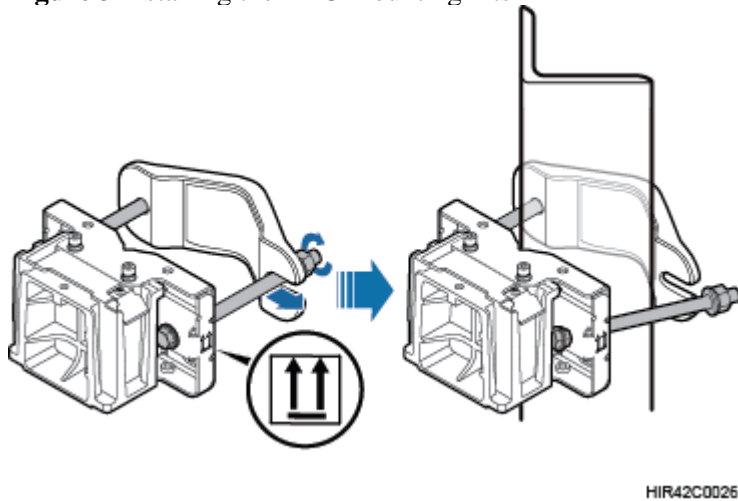
Figure 3 Installing the RRU mounting kits
