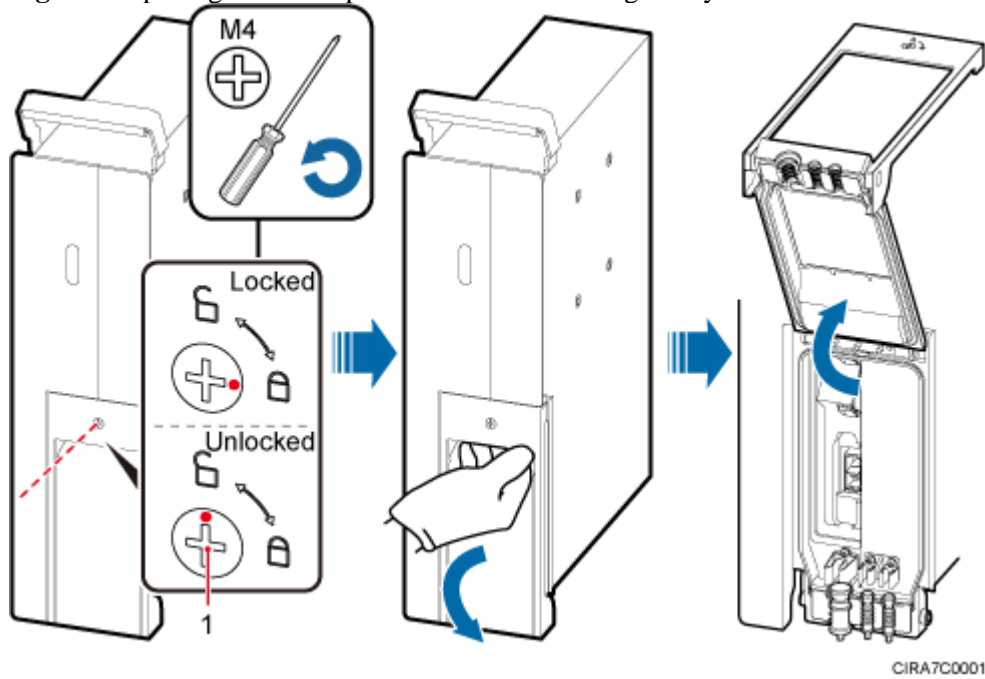
Figure 1 Opening the cover plate of the RRU cabling cavity
