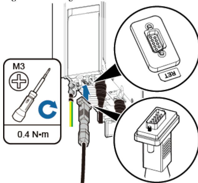
Figure 1 Installing an RRU AISG multi-wire cable
