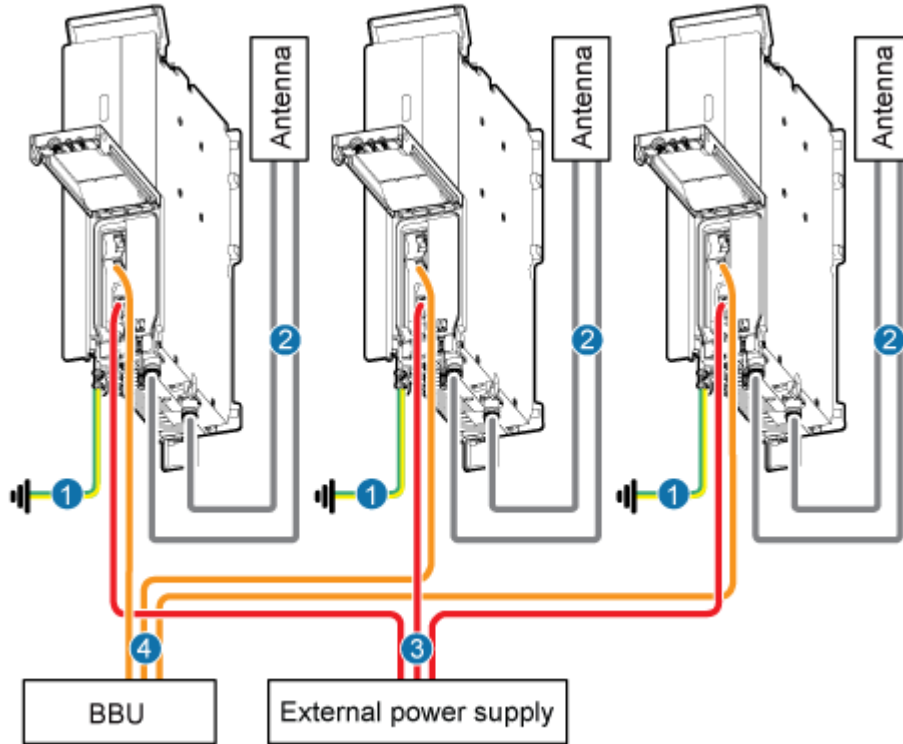
Figure 4 Cable connections of multiple single-mode RRUs
