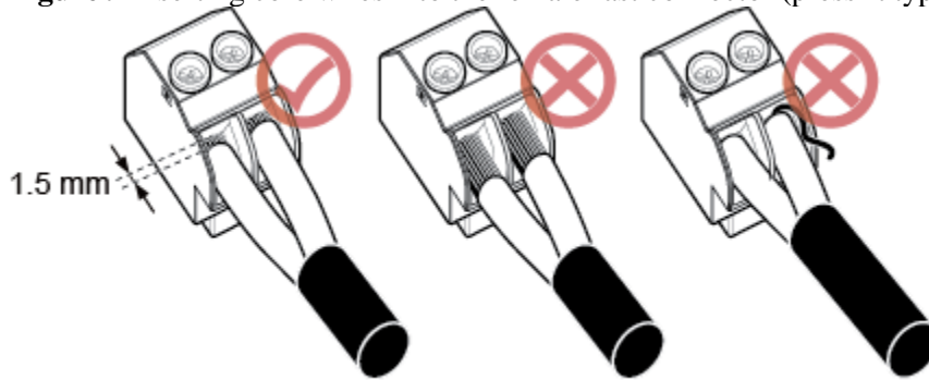
Figure 9 Inserting core wires into the female fast connector (pressfit type)
