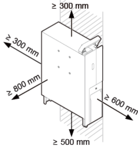
Figure 2 Clearance for a single RRU in standard or reverse mode Recommended Clearances
