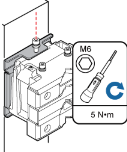
Figure 5 Securing the captive screw into the connection hole
