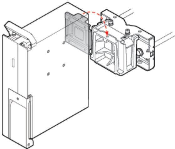
Figure 4 Installing the RRU onto the main bracket
