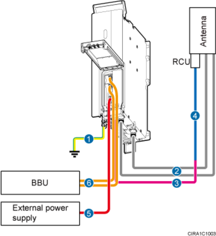
Figure 3 Cable connections of a multimode RRU
