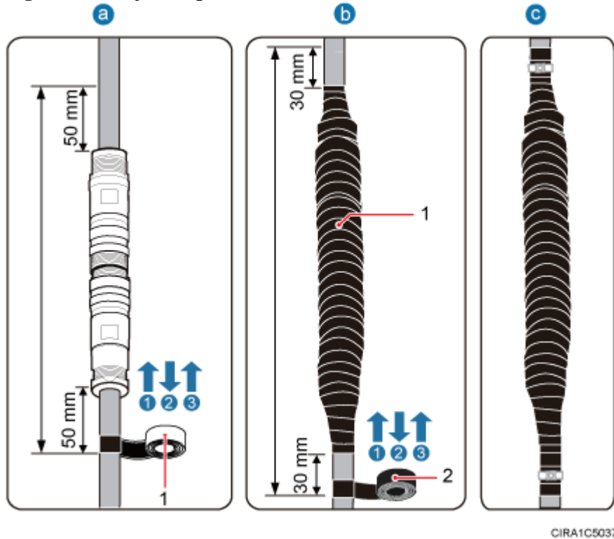
Figure 4 Waterproofing the connector on the AISG multi-wire cable
