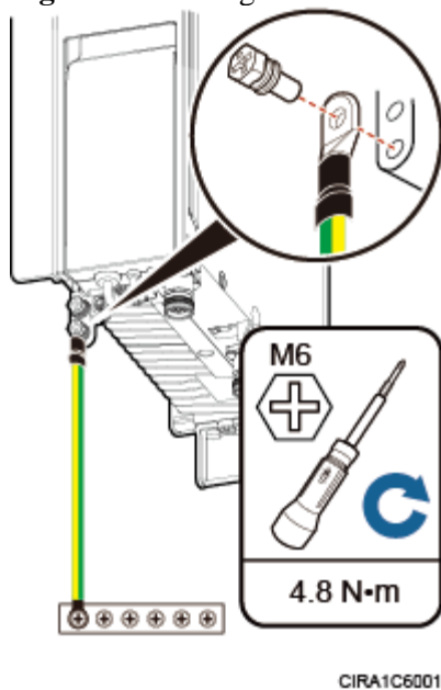
Figure 1 Installing an RRU PGND cable
