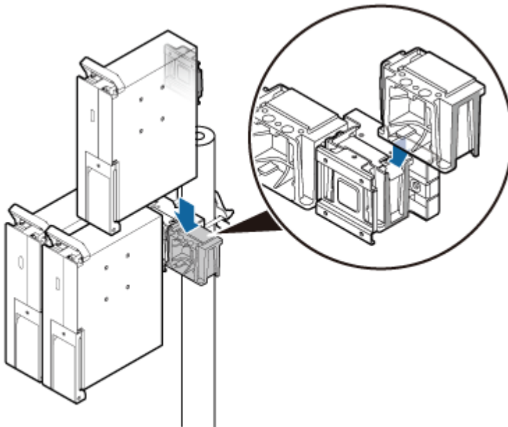
Figure 3 Installing the third RRU onto the third main bracket
