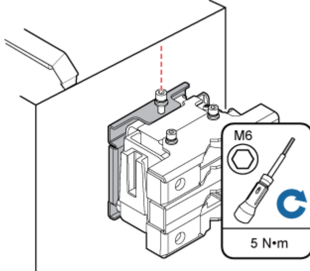
Figure 8 Securing the captive screw into the connection hole
