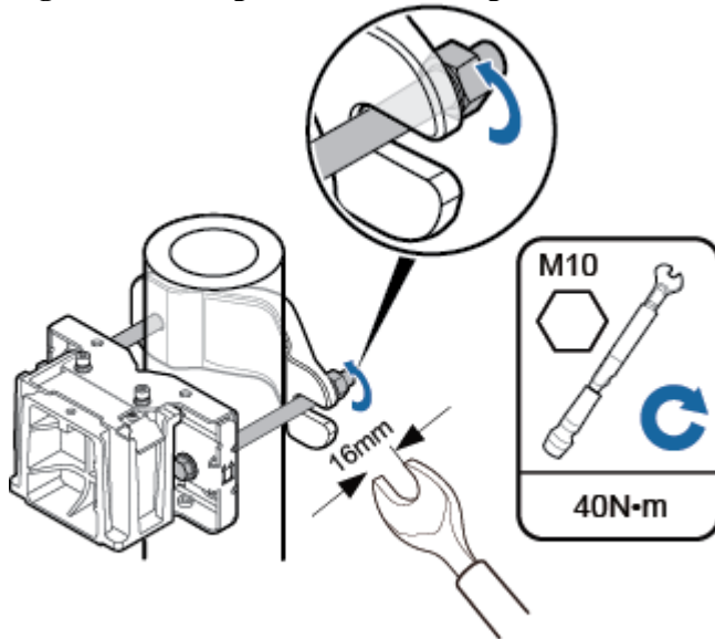
Figure 3 Securing the RRU mounting kits
