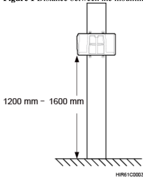
Figure 1 Distance between the mounting kits and the ground
