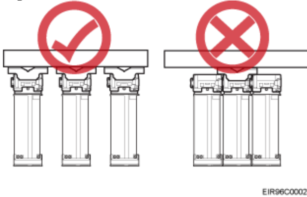
Figure 13 Correct installation of RRUs installed on a wall in side-mounted mode
