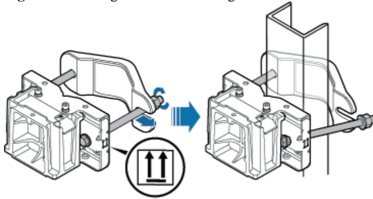
Figure 3 Installing the RRU mounting kits
