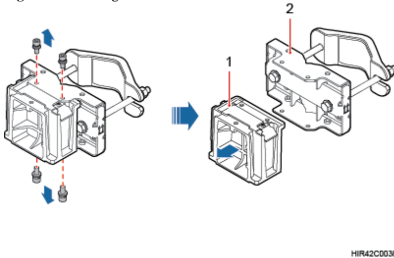
Figure 2 Removing the RRU main bracket
