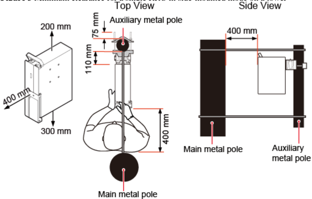
Figure 3 Minimum clearance for a single RRU in side-mounted mode on a tower
