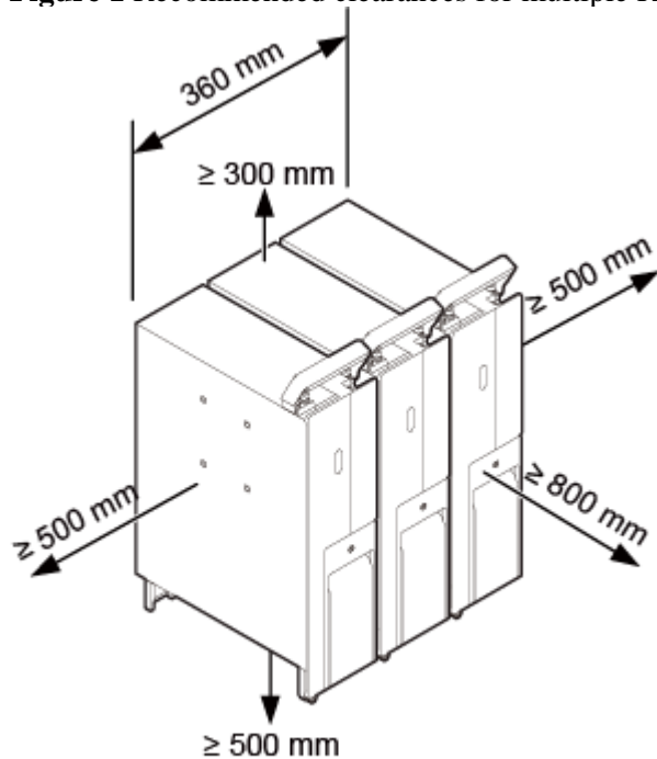
Figure 1 Recommended clearances for multiple RRUs installed in stacked mode
