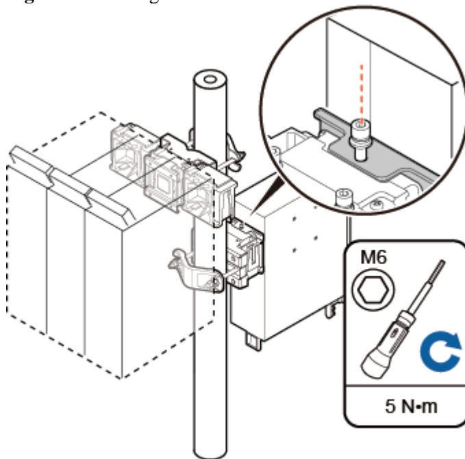
Figure 7 Installing the fourth RRU onto the fourth main bracket
