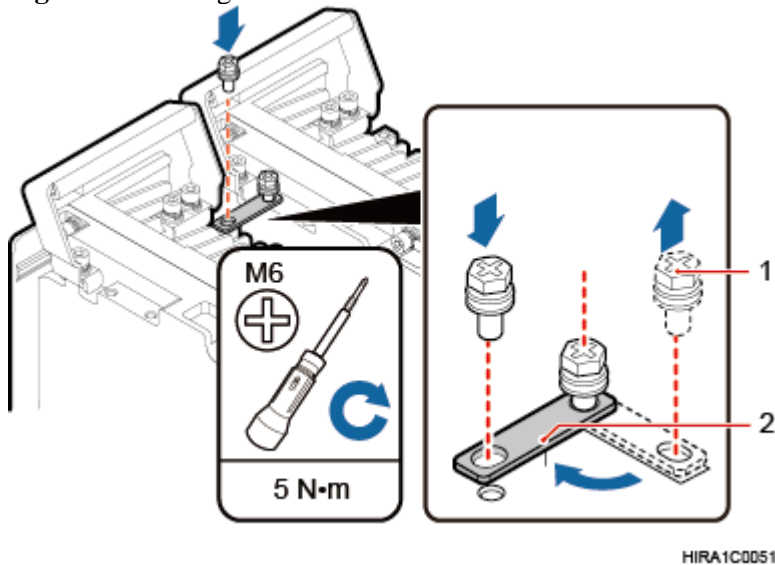
Figure 5 Installing the sheet metal tab
