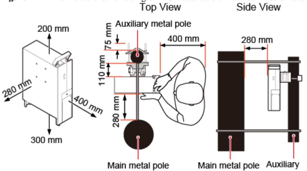
Figure 4 Minimum clearance for a single RRU in standard or reverse mode on a tower
