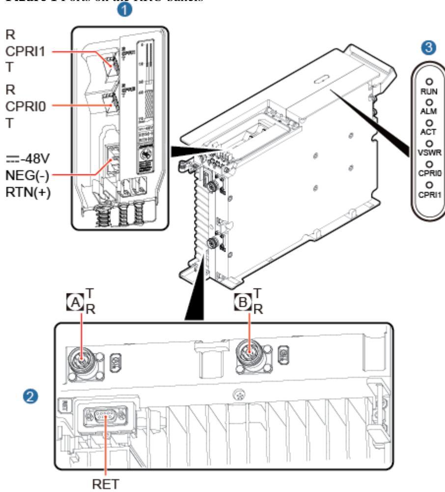
Figure 1 Ports on the RRU panels
