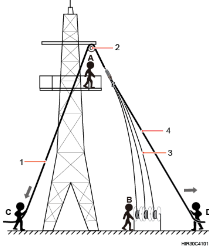
Figure 1 Hoisting optical fibers onto the tower
