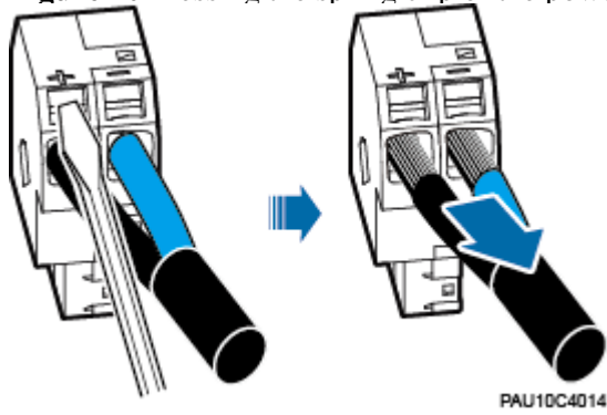
Figure 10 Pressing the spring clip of the power terminal
