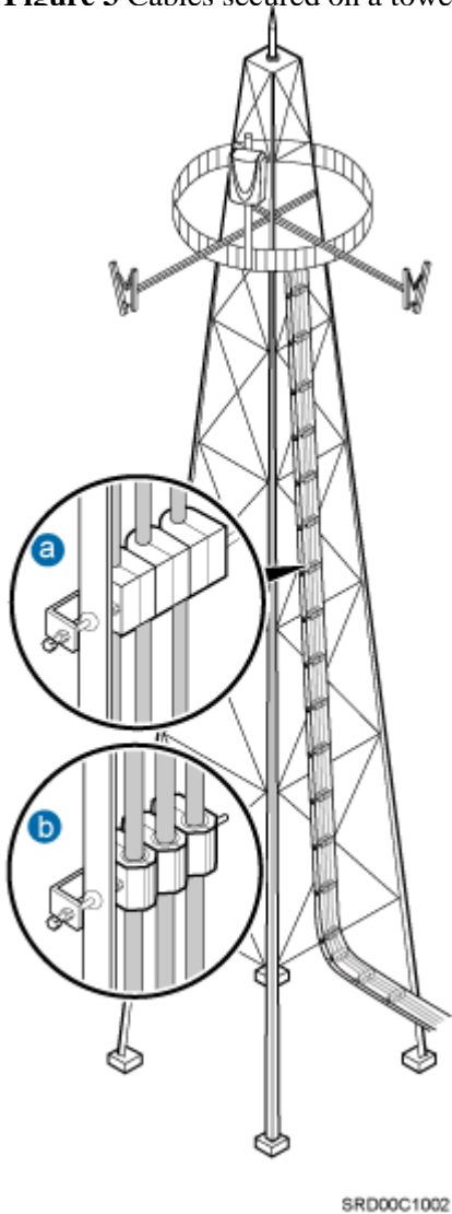
Figure 3 Cables secured on a tower
