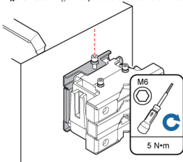
Figure 7 Securing the captive screw into the connection hole
