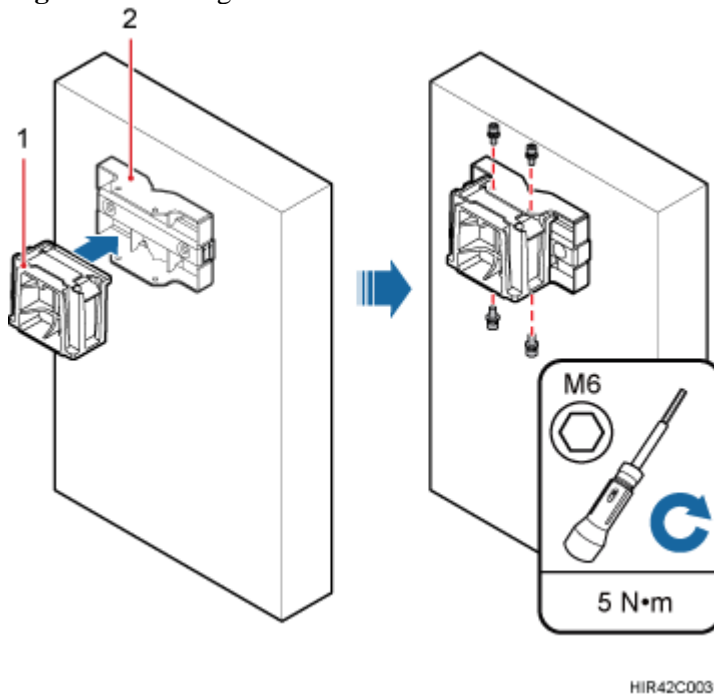
Figure 5 Installing the main bracket
