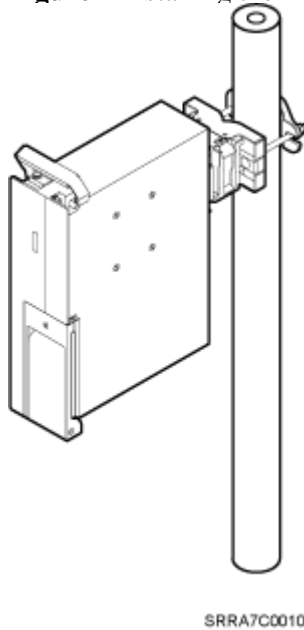
Figure 1 Installing the first RRU onto the main bracket
