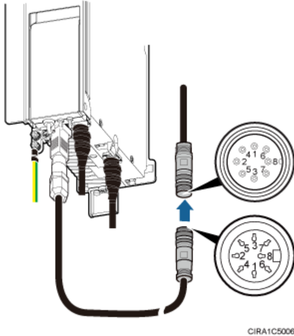
Figure 2 Installing an RRU AISG multi-wire cable
