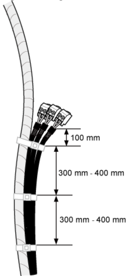
Figure 2 Binding cable ties
