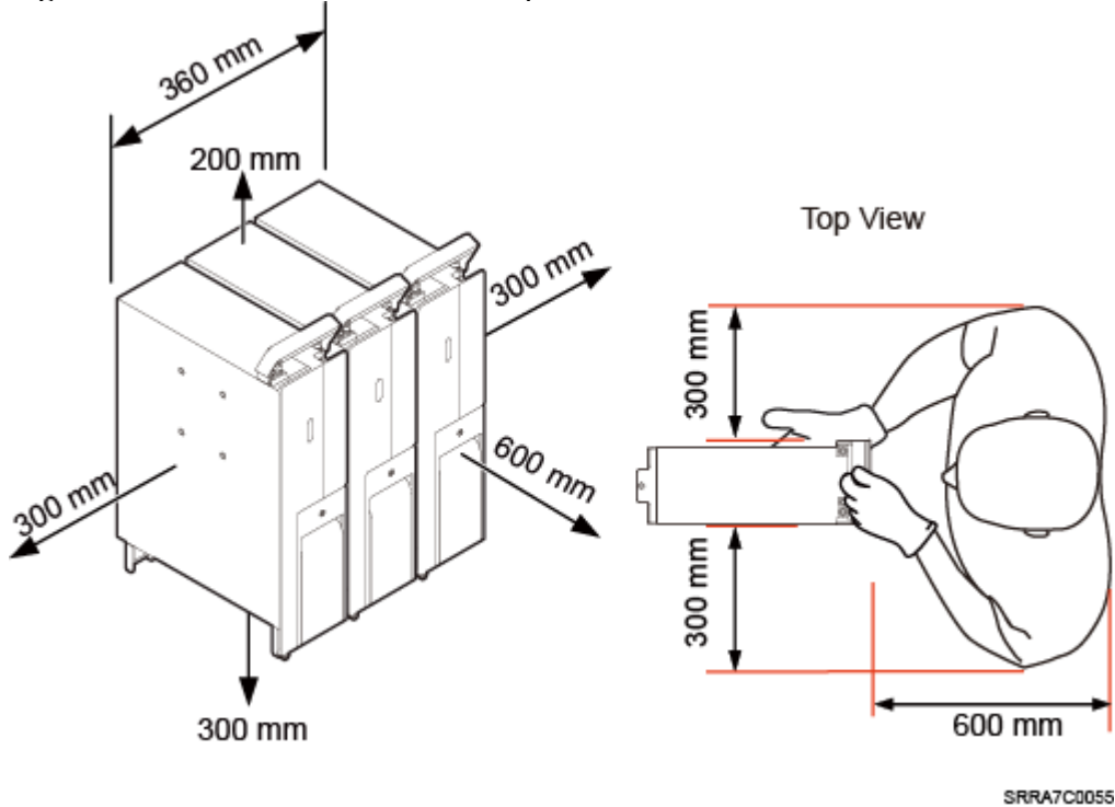
Figure 2 Minimum clearances for multiple RRUs installed in stacked mode
