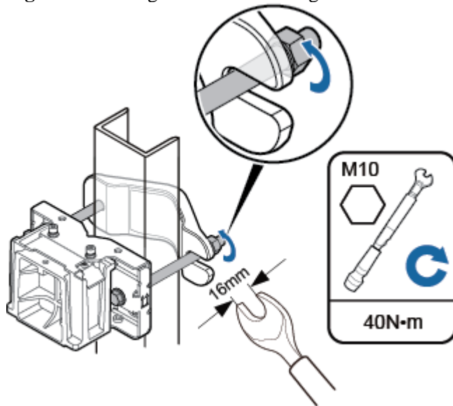
Figure 4 Securing the RRU mounting kits
