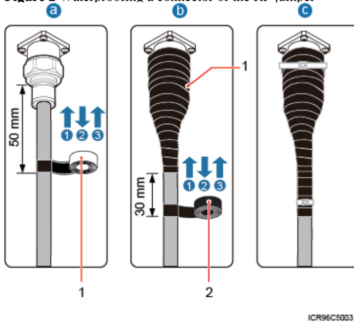
Figure 2 Waterproofing a connector of the RF jumper
