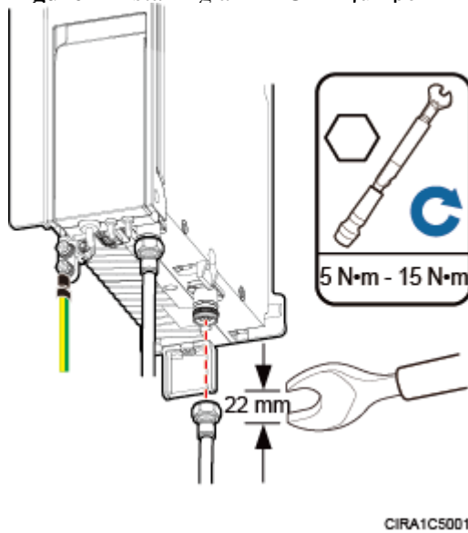
Figure 1 Installing an RRU RF jumper
