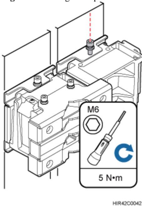
Figure 6 Securing the captive screw into the connection hole
