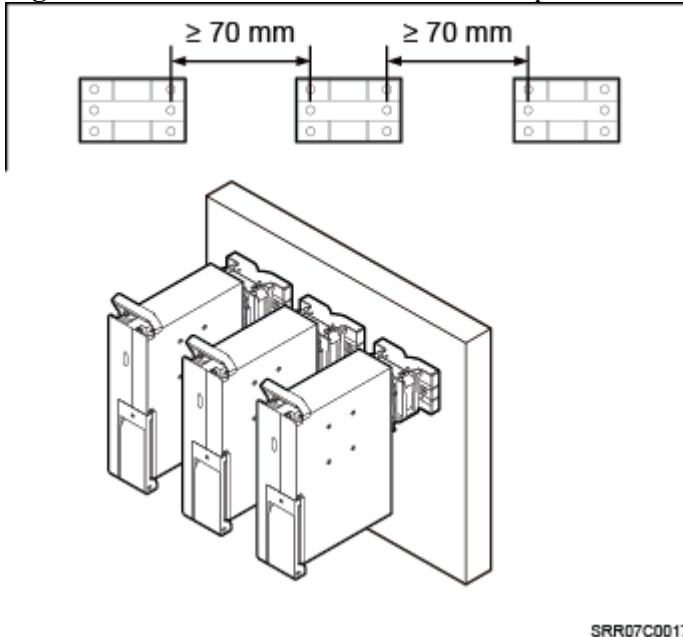
Figure 5 Recommended clearances for multiple RRUs installed in side-mounted mode on a wall
