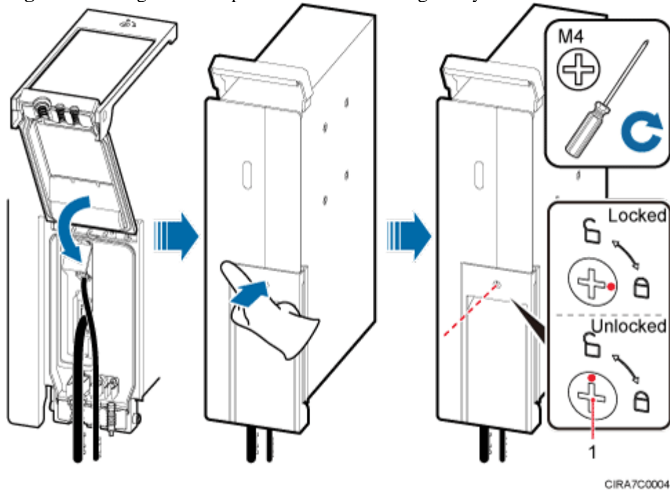
Figure 3 Closing the cover plate of an RRU cabling cavity
