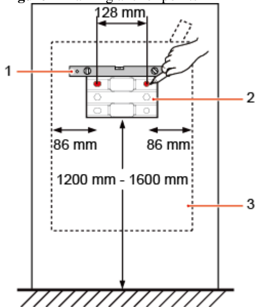
Figure 2 Marking anchor points
