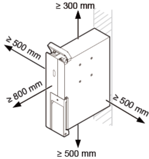
Figure 1 Clearance for a single RRU in side-mounted mode Recommended Clearances
