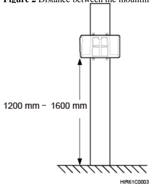
Figure 2 Distance between the mounting kits and the ground
