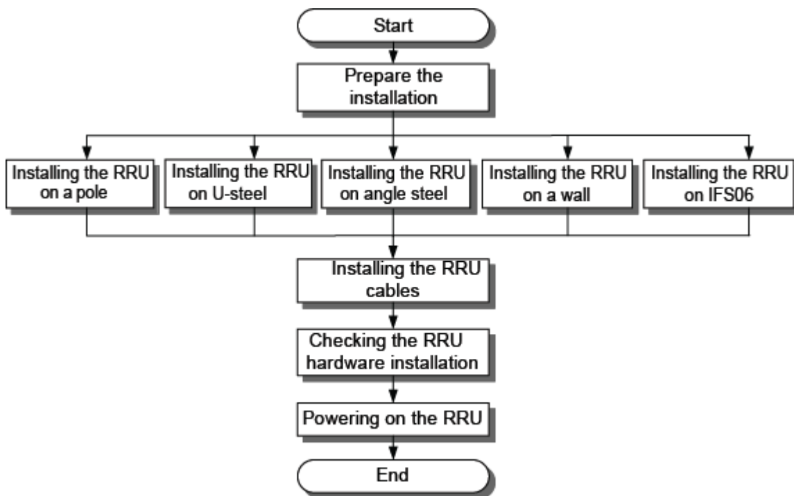
Figure 1 Process of installing an RRU
