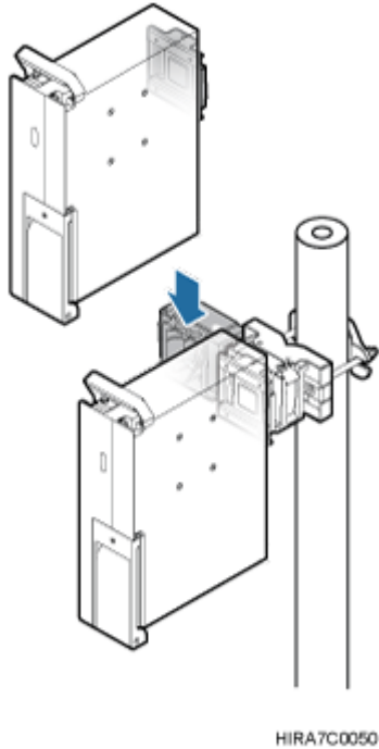
Figure 5 Installing the second RRU onto the main bracket
