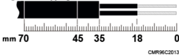
Figure 5 Matched length
