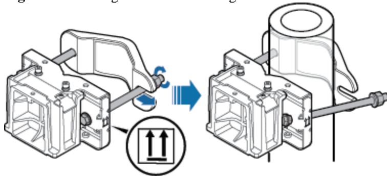
Figure 2 Installing the RRU mounting kits
