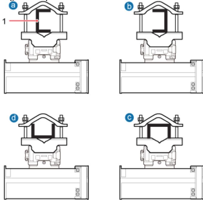
Figure 1 Top view of an RRU
