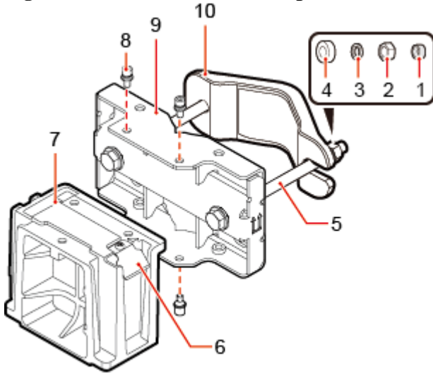
Figure 2 12 L blade RRU mounting kit
