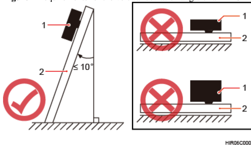
Figure 2 Requirements for the vertical deviation angle of an RRU
