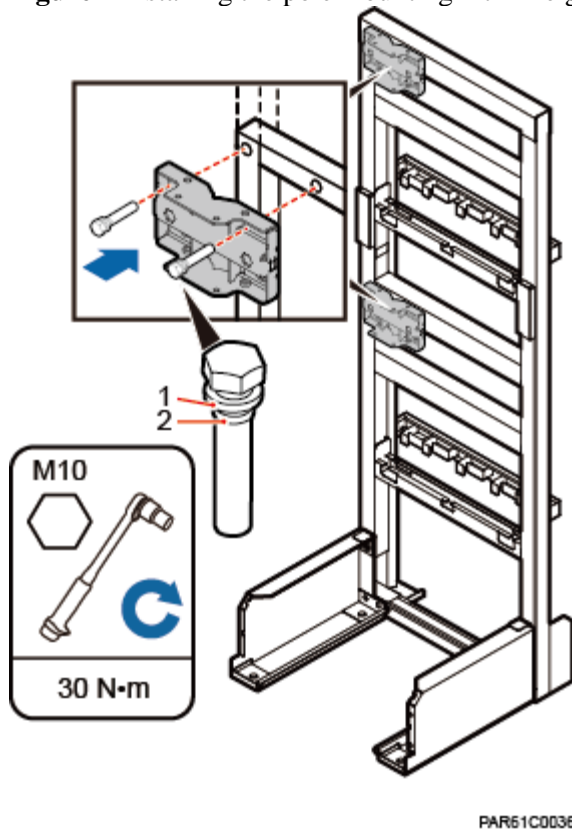
Figure 2 Installing the pole mounting kit in height-unrestricted scenario
