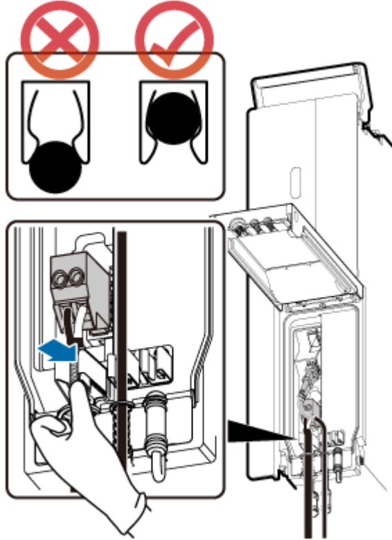
Figure 1 Fastening cables using clips
