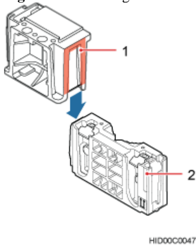
Figure 4 Connecting to the main mounting bracket for installing a common RRU
