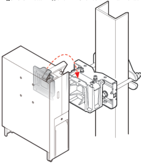
Figure 6 Installing the RRU onto the main brackets
