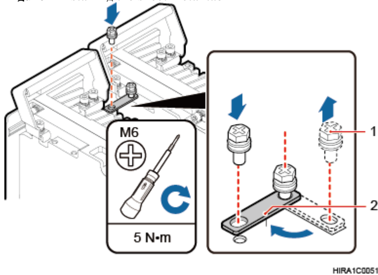
Figure 7 Installing the sheet metal tab
