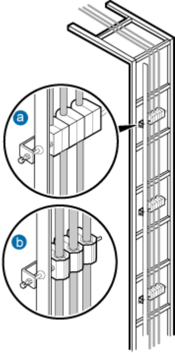
Figure 2 Cables secured on a cable tray
