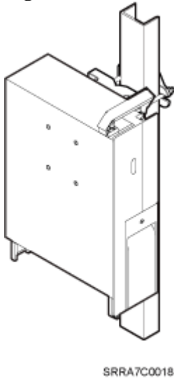
Figure 10 RRU installed on U-steel
