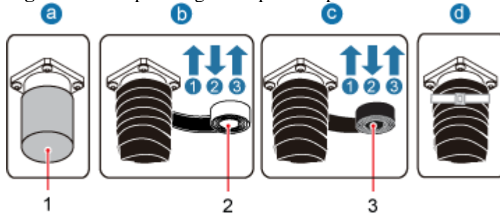
Figure 3 Waterproofing a dustproof cap
