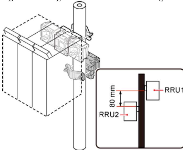
Figure 6 Installing the second set of RRU mounting kits
