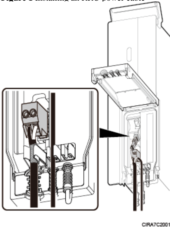
Figure 1 Installing an RRU power cable
