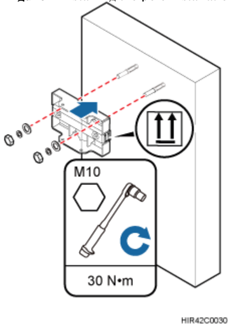
Figure 4 Installing the pole installation bracket on the expansion anchor bolts
