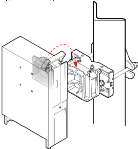
Figure 6 Installing the RRU onto the main brackets
