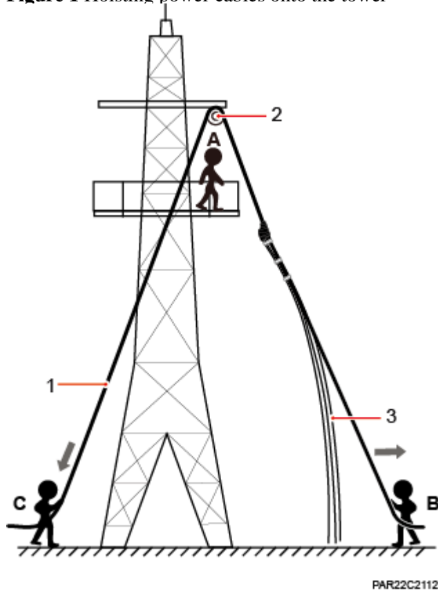
Figure 1 Hoisting power cables onto the tower
