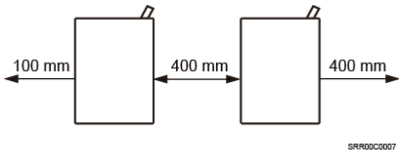
Figure 2 Minimum horizontal spacing between RRUs
