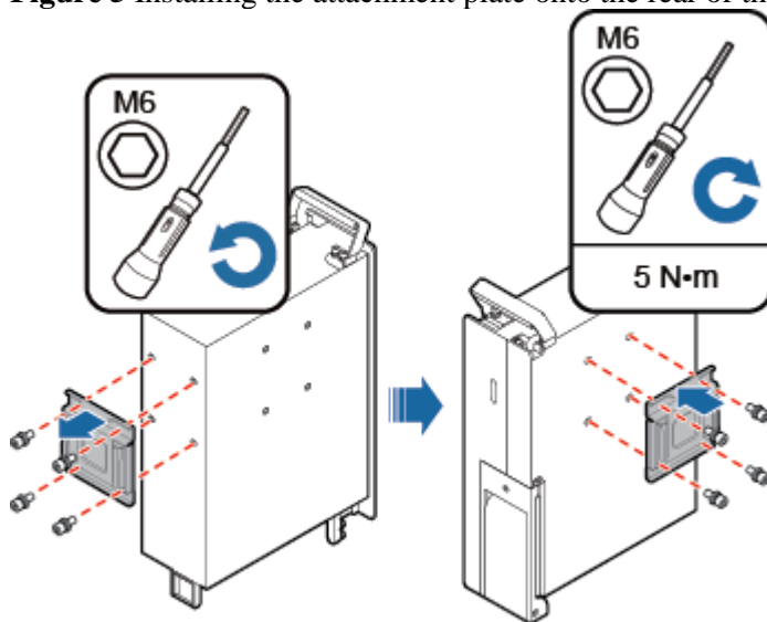
Figure 5 Installing the attachment plate onto the rear of the RRU
