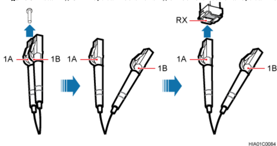
Figure 3 Installing CPRI optical fibers for single-fiber bidirectional optical modules
