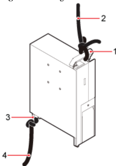
Figure 2 Binding the RRU
