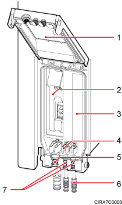
Figure 2 RRU cabling cavity
