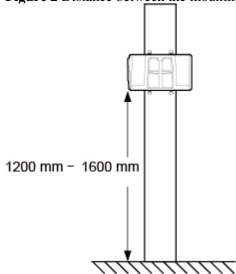
Figure 2 Distance between the mounting kits and the ground
