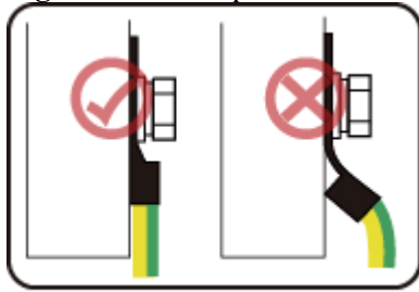
Figure 2 Correct position of an OT terminal
