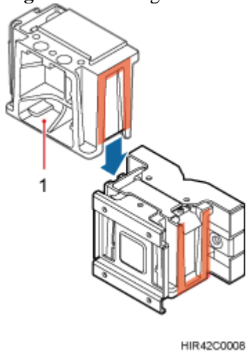
Figure 3 Installing the second main bracket
