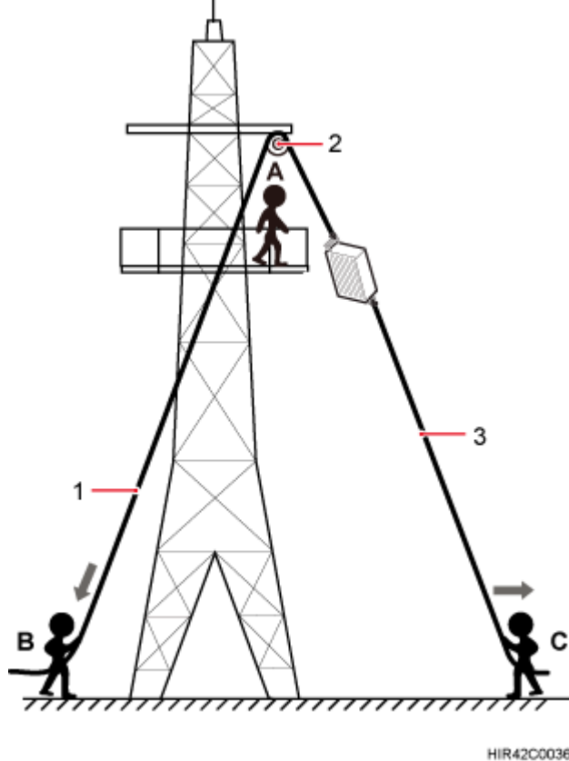
Figure 5 Hoisting the RRU onto the tower
