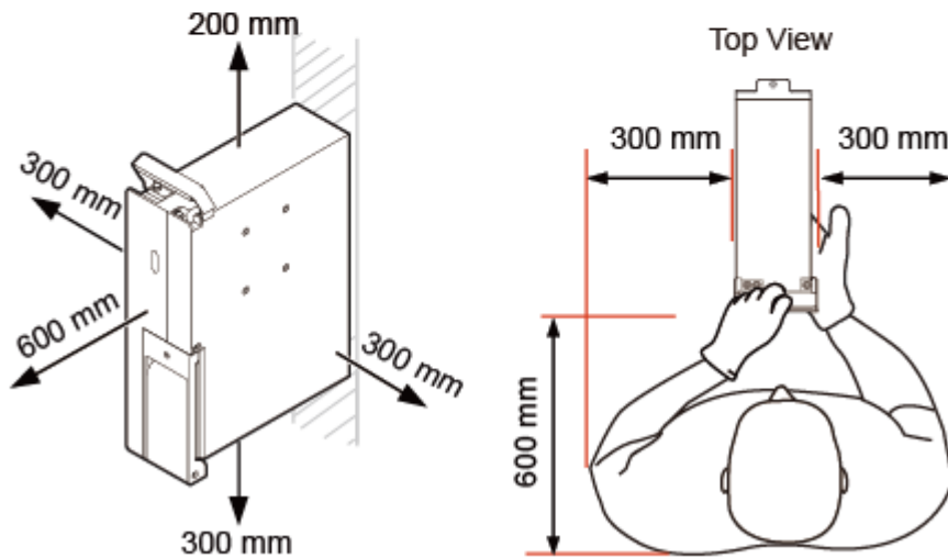
Minimum Clearances
