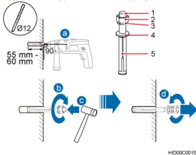
Figure 3 Drilling holes and inserting expansion anchor bolts
