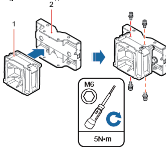
Figure 3 Installing the RRU main brackets
