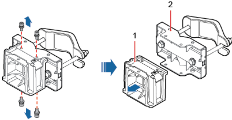
Figure 2 Removing the RRU main bracket
