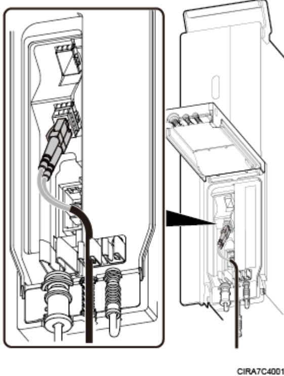
Figure 2 Installing CPRI optical fibers for dual-fiber bidirectional optical modules
