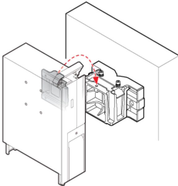
Figure 7 Installing the RRU onto the main bracket
