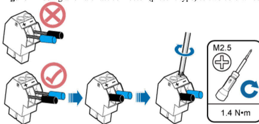
Figure 7 Adding a female fast connector (pressfit type) to two core wires
