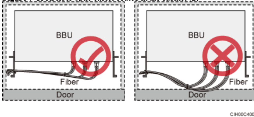
Figure 8 FE/GE fiber optic cables routed in the cabinet
