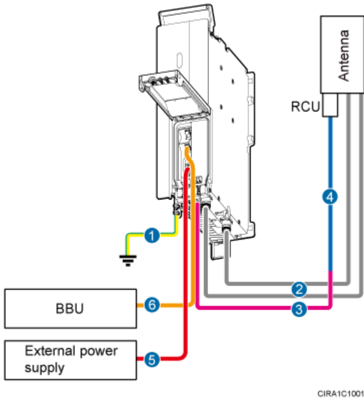
Figure 1 Cable connections of a single-mode RRU (MEB not installed)
