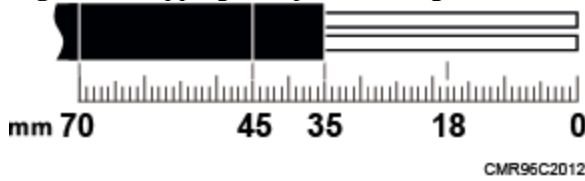
Figure 3 Stripping the specified length of sheath
