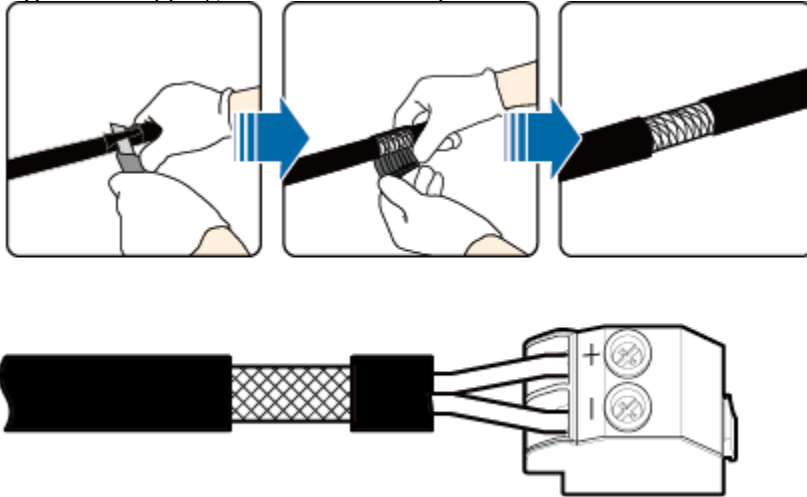
Figure 8 Stripping the sheath off the power cable
