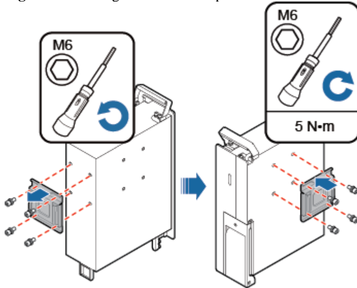
Figure 6 Installing the attachment plate onto the rear of the RRU
