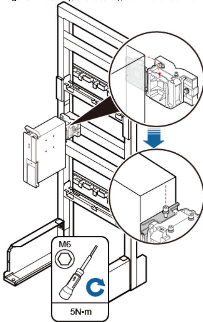
Figure 4 Installing and securing the RRU on the main bracket
