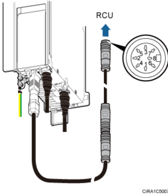
Figure 3 Installing an RRU AISG extension cable
