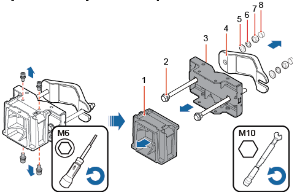
Figure 1 Disassembling the RRU mounting kits
