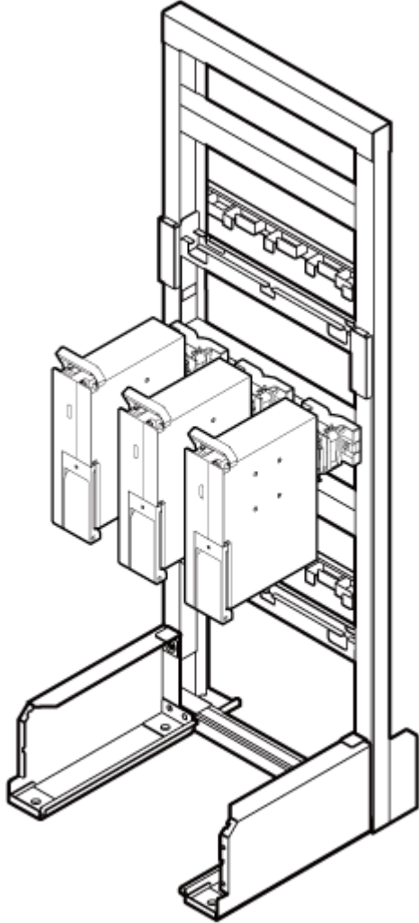
Figure 5 Installing RRUs on the lower level
