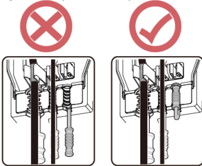
Figure 2 Correct placement of waterproof blocks
