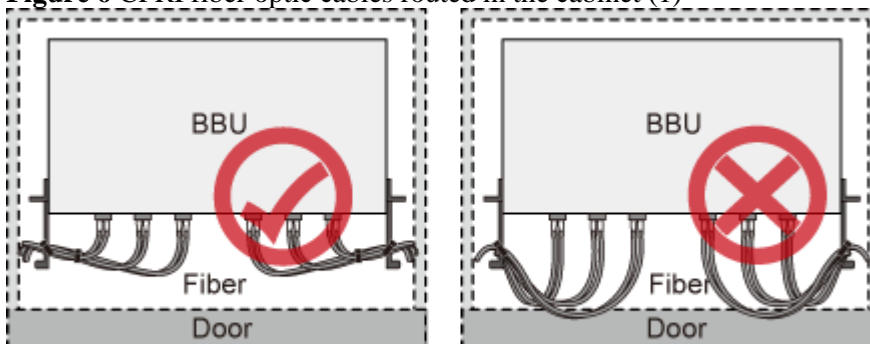
Figure 6 CPRI fiber optic cables routed in the cabinet (1)
