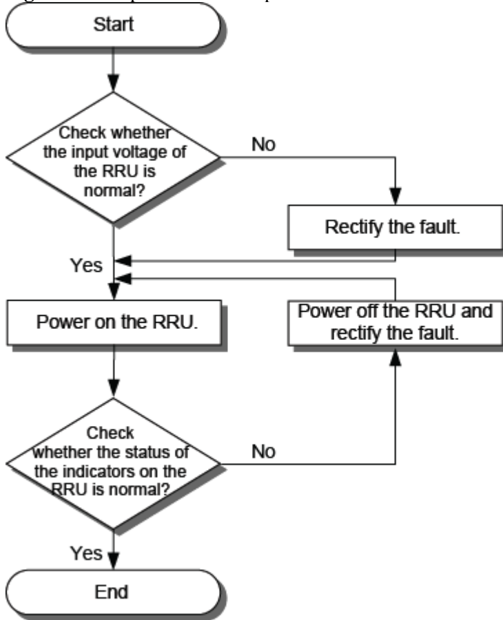
Figure 1 RRU power-on check process
