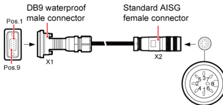
Figure 3-13 AISG multi-wire cable
