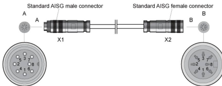
Figure 3-14 AISG extension cable
