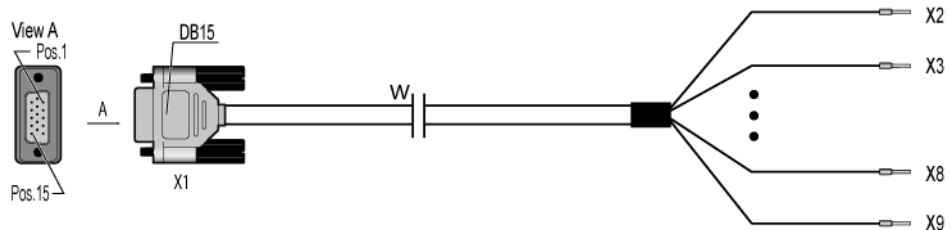
Figure 3-10 Alarm cable
