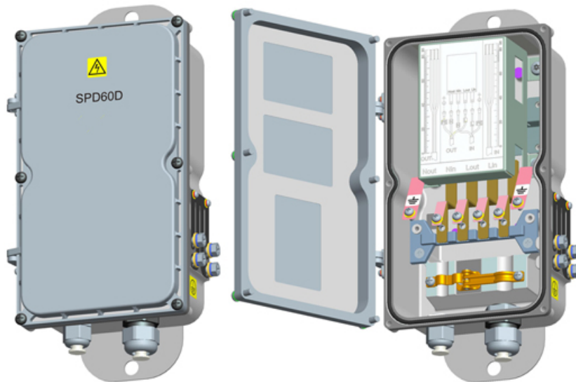
Figure 4-1 AC power surge protection box
