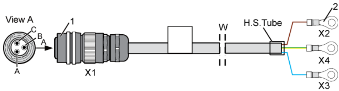
Figure 3-5 Power cable between the AC RRU and the AC surge protection box
