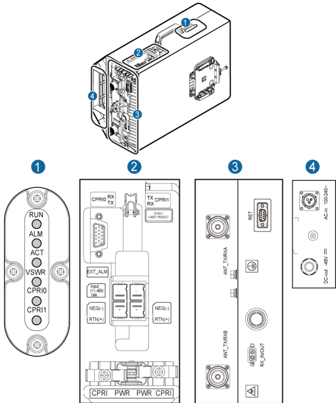
Figure 2-4 Panels of the AC RRU
