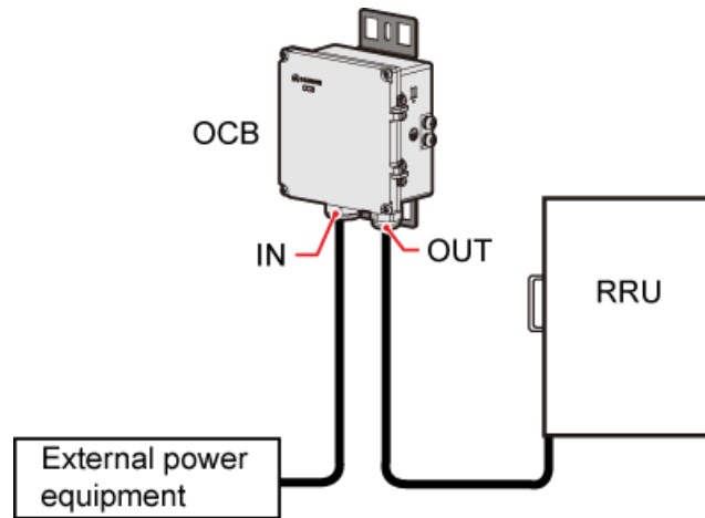
Figure 4-4 The application scenario of the OCB
