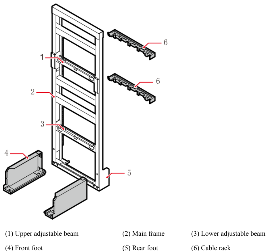
Figure 4-3 Structure of the IFS06
