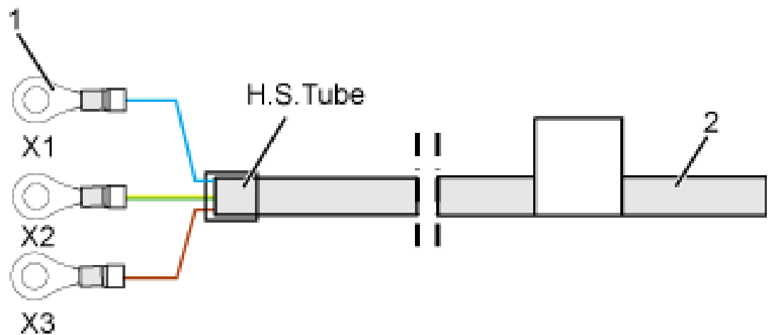
Figure 3-6 Power cable between the AC surge protection box and the external power equipment
