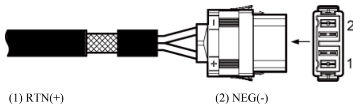
Figure 3-3 Power cable for the DC RRU
