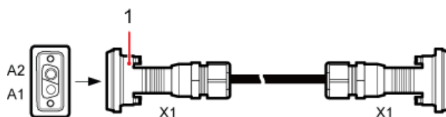
Figure 3-12 Interconnect jumper
