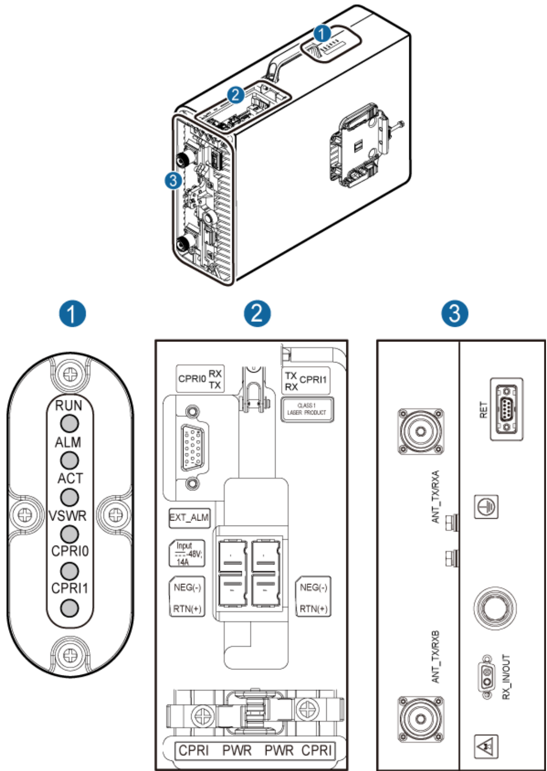
Figure 2-3 Panels of the DC RRU
