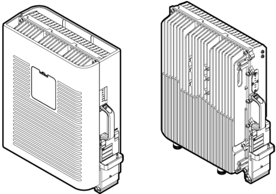
Figure 2-1 DC RRU
